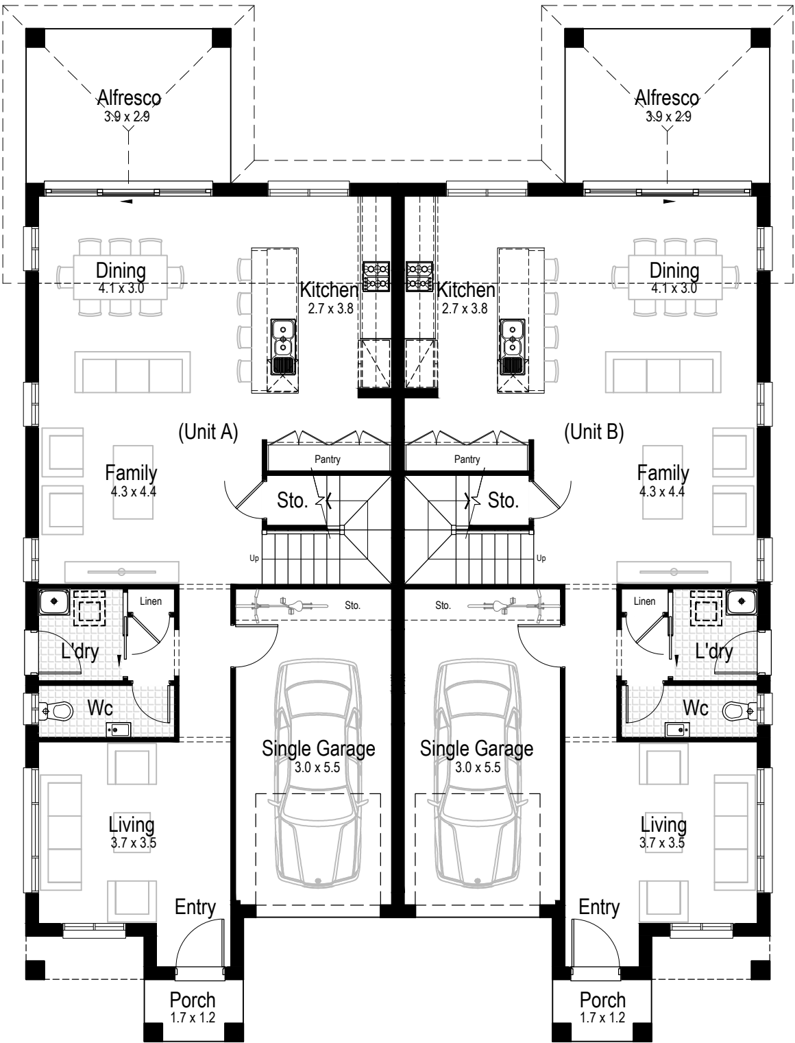
Ground Floor
